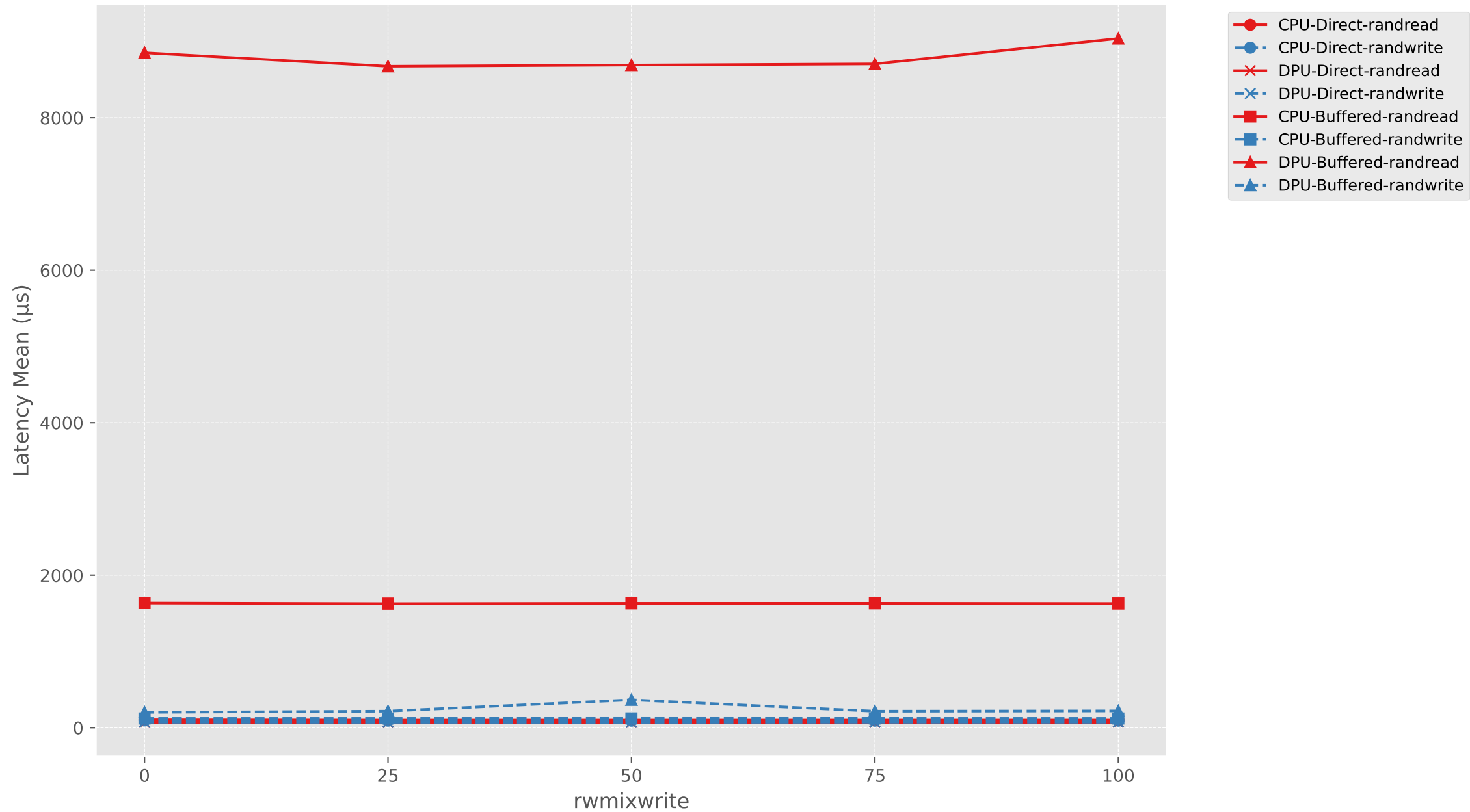
Latency Mean vs rwmixwrite (CPU vs DPU, Direct vs Buffered)
